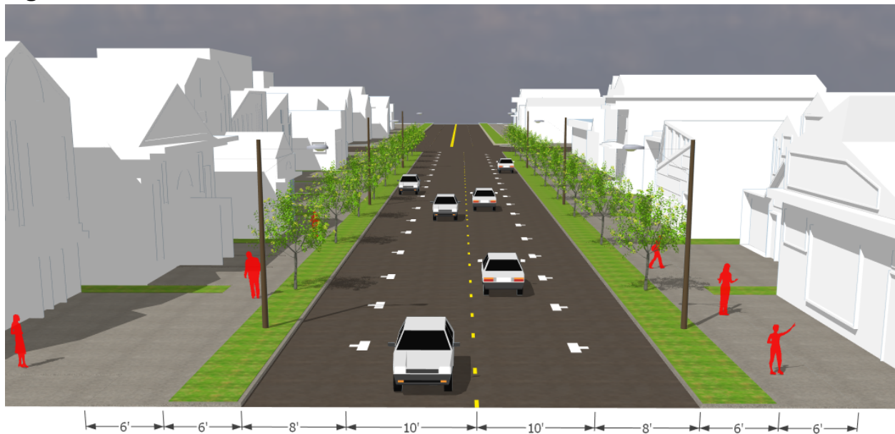
Figure 10. Local Street Standard
